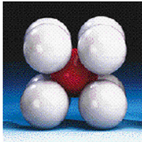
body-centered cubic
